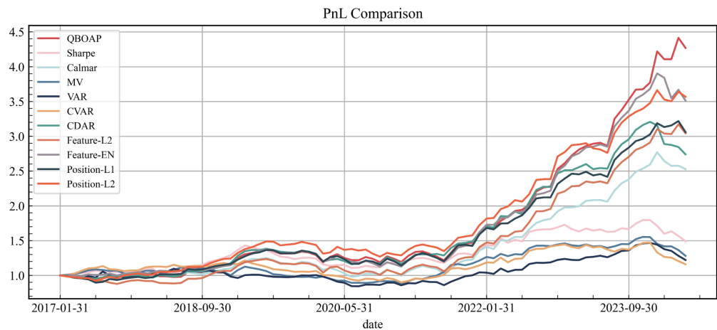
Figure 2: Pnl Comparison of QBOAP framework and Baseline
